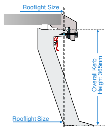
Figure 7: rooflight with 300mm PVC kerb detail
